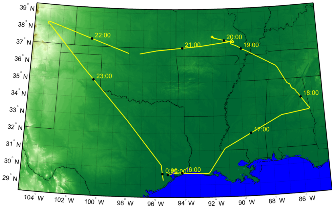
Figure 1. DC-8 flight track for September 6, 2013.
