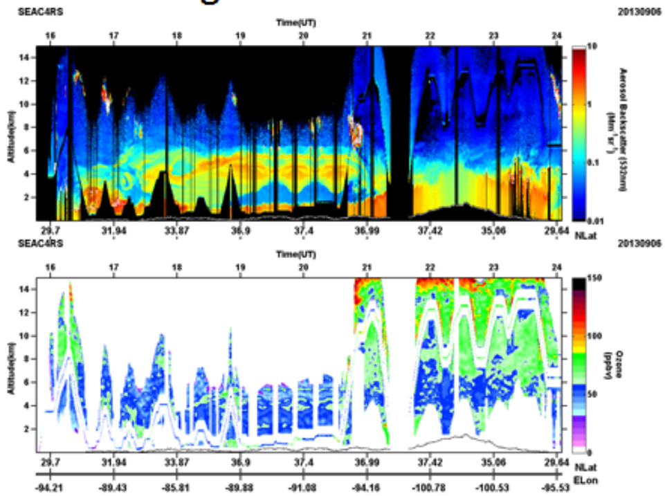
Figure 2. DIAL/HSRL aerosol backscatter and ozone mixing ratio curtains along the September 6, 2013 DC-8 flight track.
